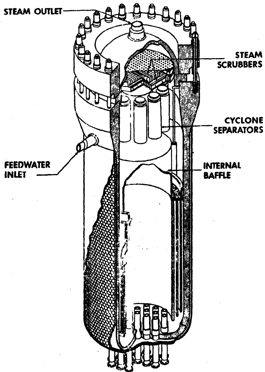
BOILING WATER REACTOR
