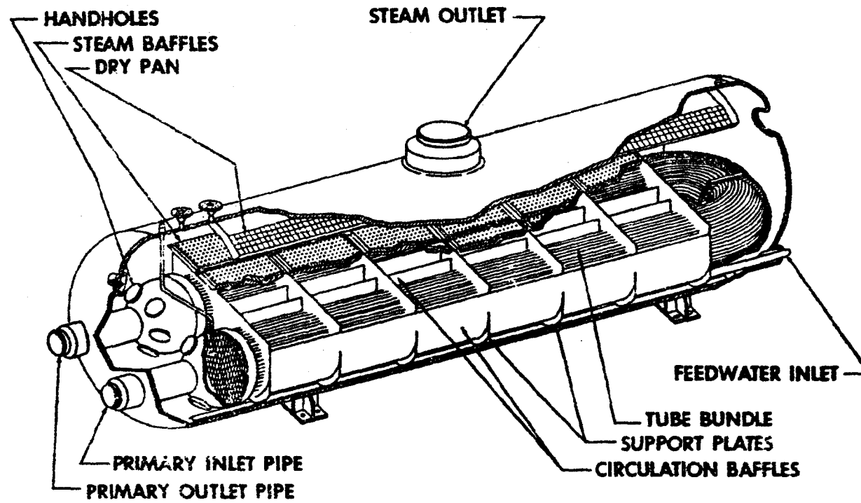
HORIZONTAL INTEGRAL DRUM BOILER
