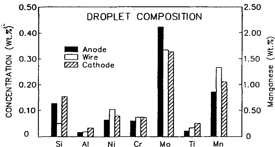
Fig. 6 - Average droplet compositions for silicon, aluminum, nickel, chromium, molybdenum, titanium and manganese for electrode-negative and electrode-positive polarities compared with the initial welding wire compositions.
