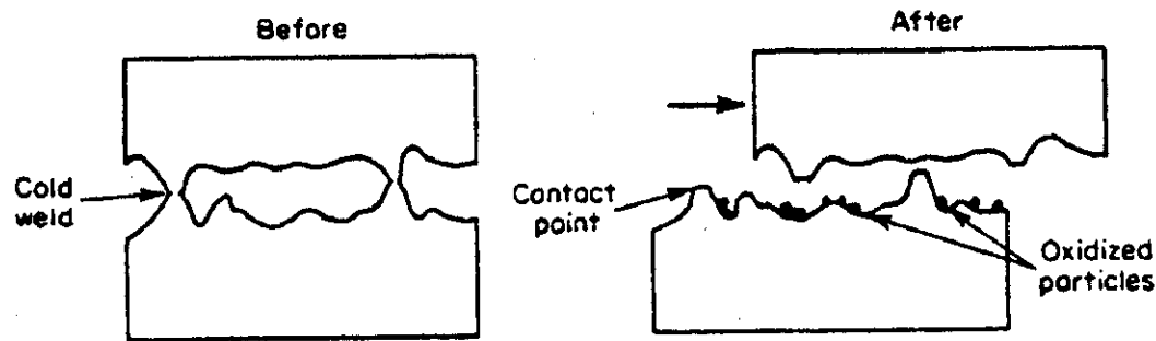
Schematic illustration of the wear-oxidation theory of fretting corrosion.
