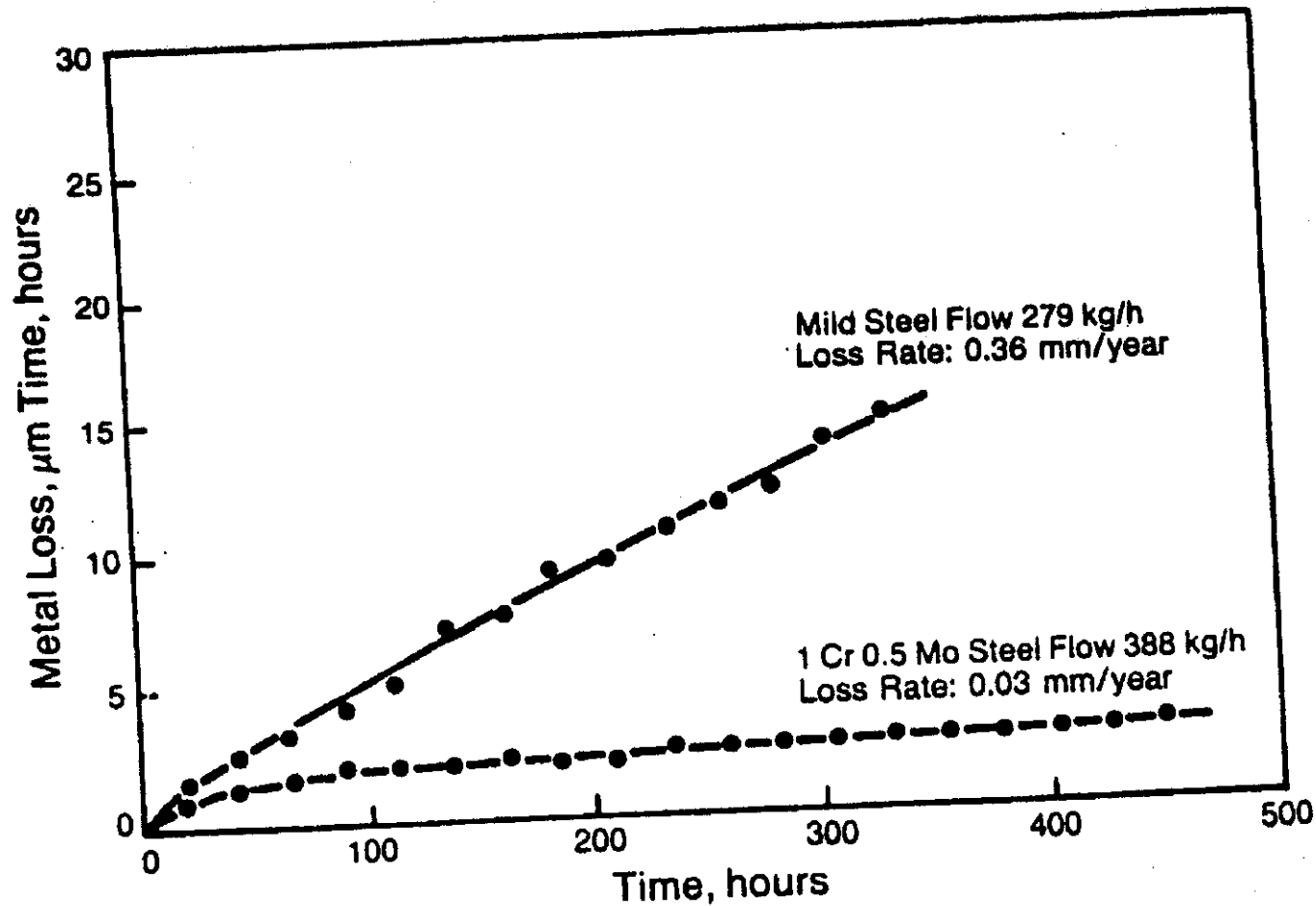
Erosion-corrosion loss as a function of time for mild steel and 1 Cr 0.5 Mo steel in water ( \text{pH}_{25} = 9.05 ) flowing through an orifice at 130^{\circ}\text{C} .
