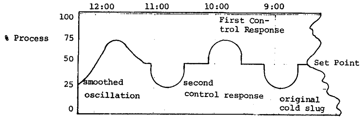
Figure 10: Chart Record of Dead Time Cycling.
